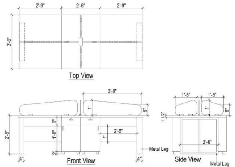
Workstation Detail Drawing
