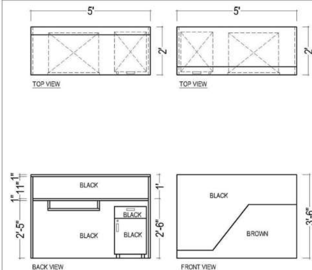
RECEPTION DESK DETAIL DRAWING 1
