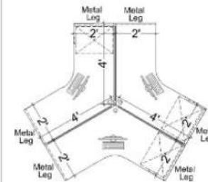
Y Shape Workstation Detail Drawing
