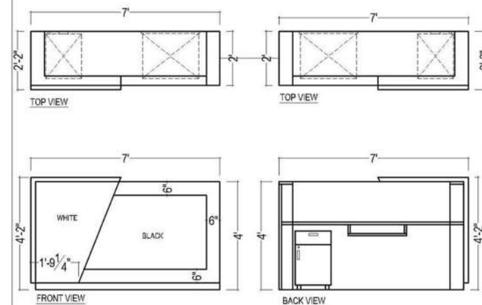
RECEPTION DESK DETAIL DRAWING 3
