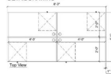
WORKSTATION DETAIL DRAWING
